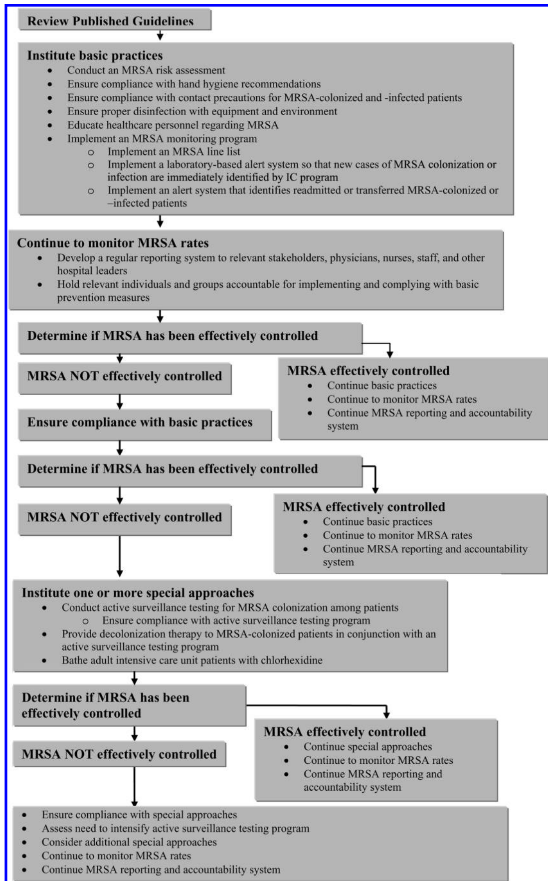
FIGURE. Approach to control and prevention of methicillin-resistant Staphylococcus aureus (MRSA) transmission. IC, infection control.
